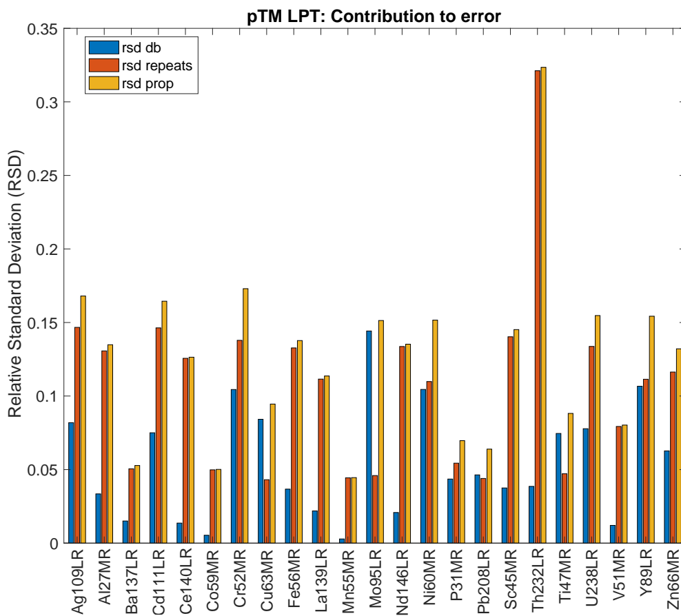
Figure 1b: Same as Figure 1a, but for the small size fraction (LPT)
